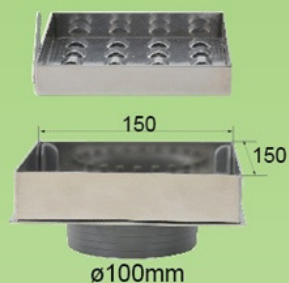
ZDL132 Shower tray waste
