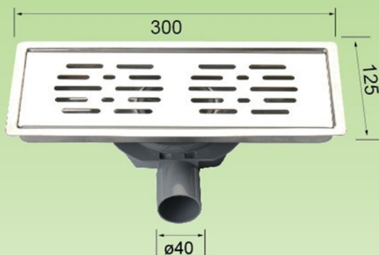
ZDL137A Showdf tray waste
