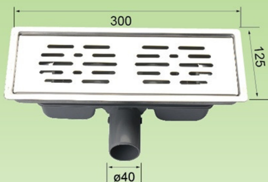
ZDL137 Showdf tray waste
