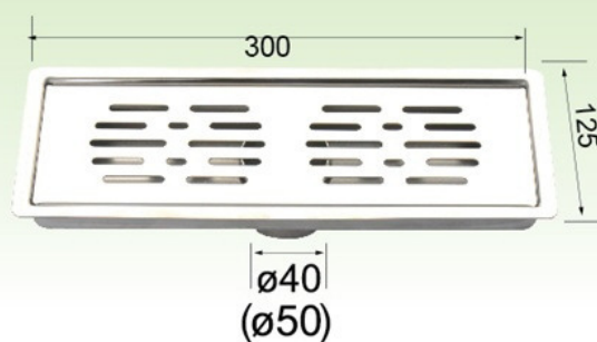
ZDL137C Showdf tray waste
